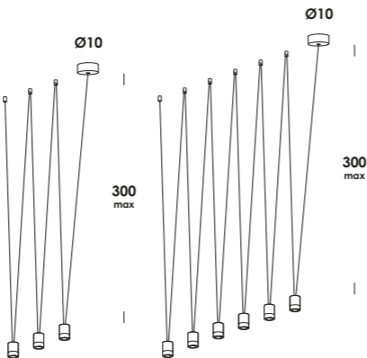
m.f.o. 10/s3 dim 3 x 3,5w 350mA 990lm 3000K - 230V fornito con driver e modulo led integrato di classe A+ luminaire contains driver and led A+
