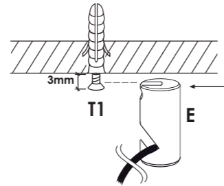
fig.1 - acc. passante cavo acc. open for cable
