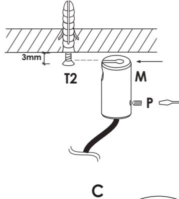
fig.2 - acc. terminale cavo acc. terminal for cable
