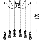
14/s6 dec. 6 E27 max 60w
