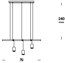
70/s3 led 3 x 3,7w 350mA 1140lm 2700k
