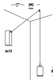
15/s2 led dec. 2 x 3,7w 350mA 760lm 2700k
