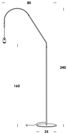
85/ph led on/off 7,5w 700mA 650lm 2700k
