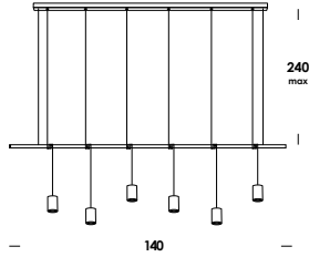
140/s6 led 6 x 3,7w 350mA 2280lm 2700k
